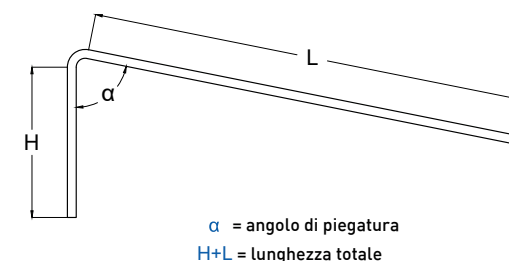
Lastre a shed Shed plates
